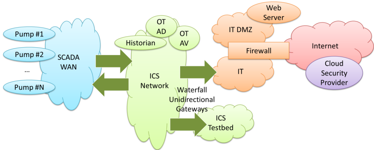
Figure (4) Modern ICS-security water treatment network proposal
