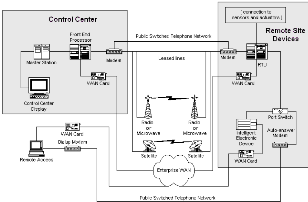
Figure C-5 Example of communication links
