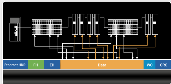
EtherCAT principle of operation
