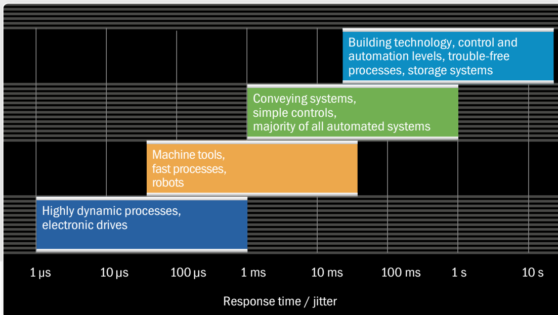
Real-time classes and application areas (IAONA classification)
