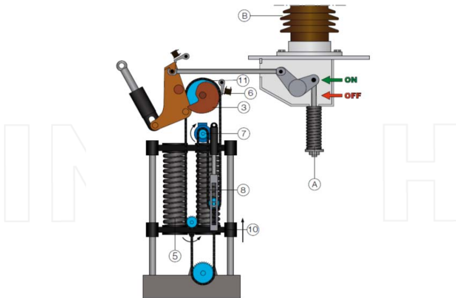
Fig. 9. Portion of HH ABB circuit breaker mechanism
