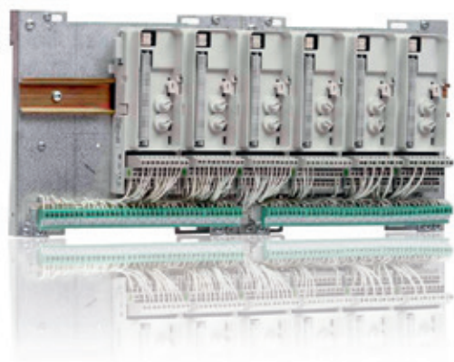
Baseplate for S400 I/O Evolution to S800 I/O
