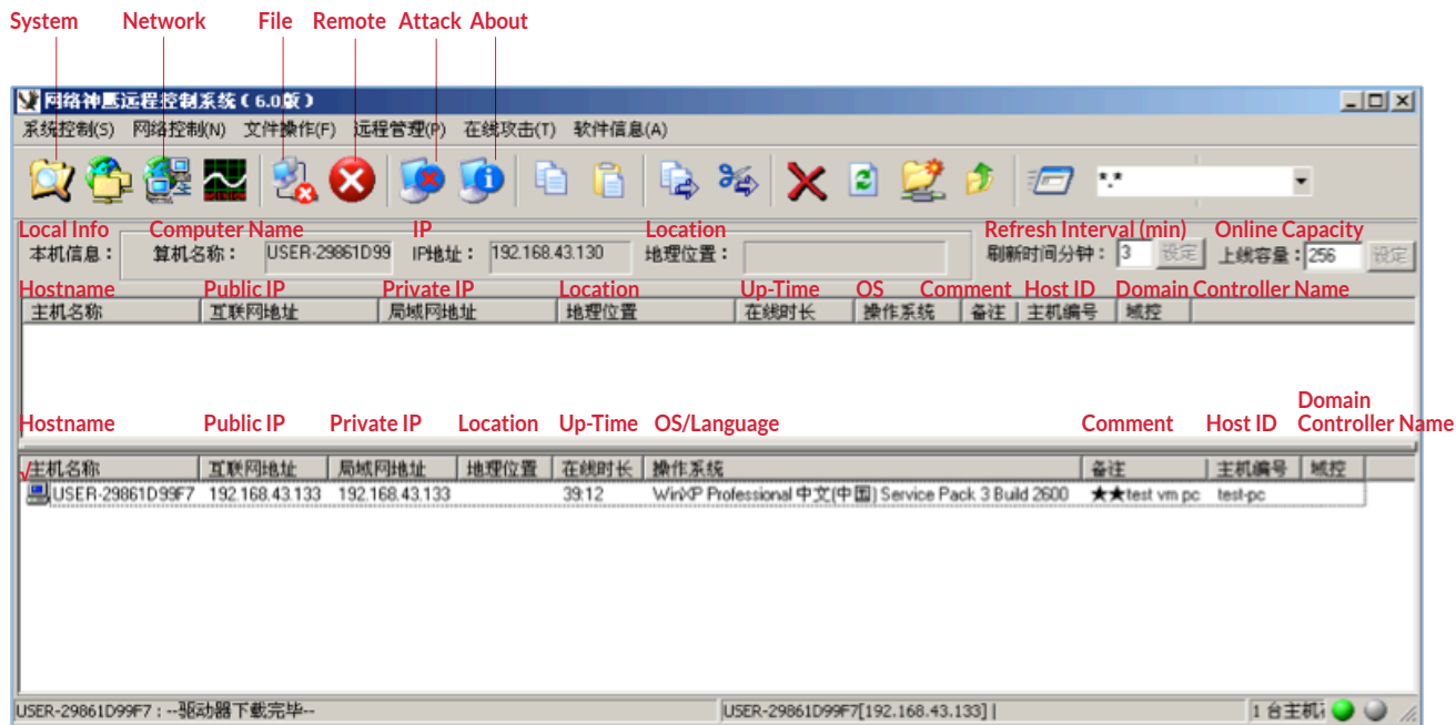
Figure 4: BACKSPACE controller GUI with sample victim data
